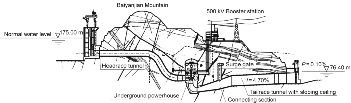
Fig. 5. Longitudinal section along the waterway system of the Three Gorges Underground Power Station. P : flood frequency; i : slope ratio.
